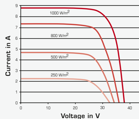
Example for AC-240P/156-60S
