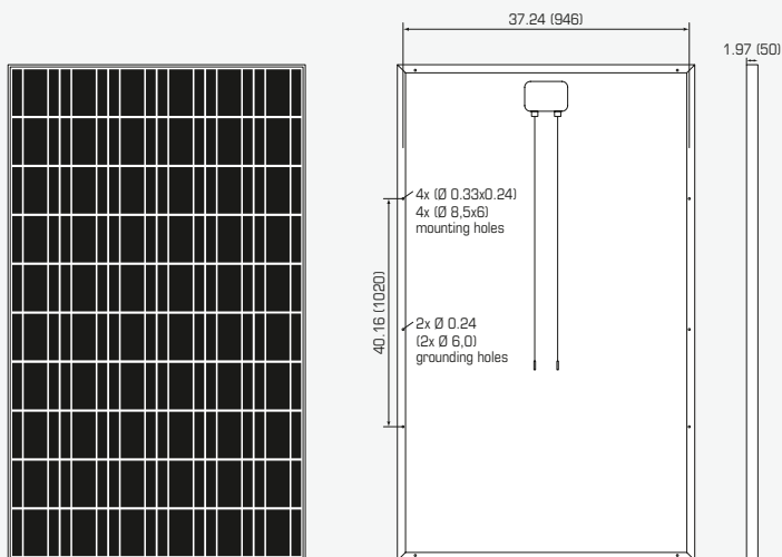
All dimensions in inch (mm)
